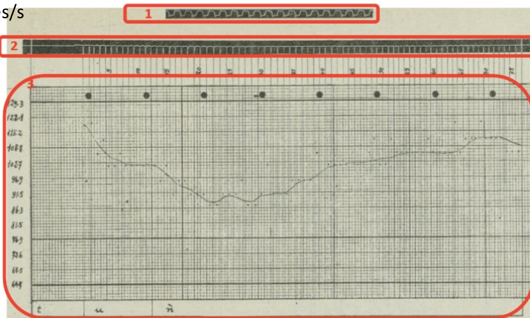
Figure 1 – Example chart of Liu's calculations of pitch values with a smoothed curve (from [23], p.19, Fig.III)
